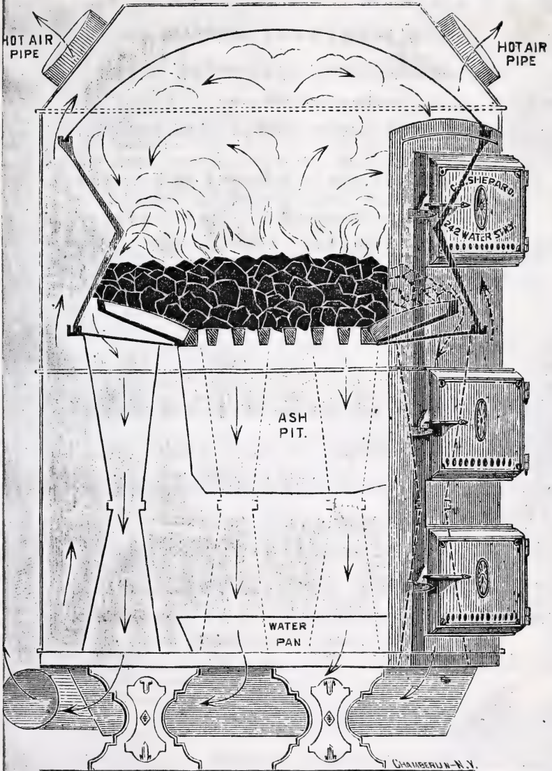
Exhibiting Fire, Combustion Chamber, Flues, Ash Pit, Evaporator, Warm Air Space. Smoke Pipe & Galvanized Iron Case.
